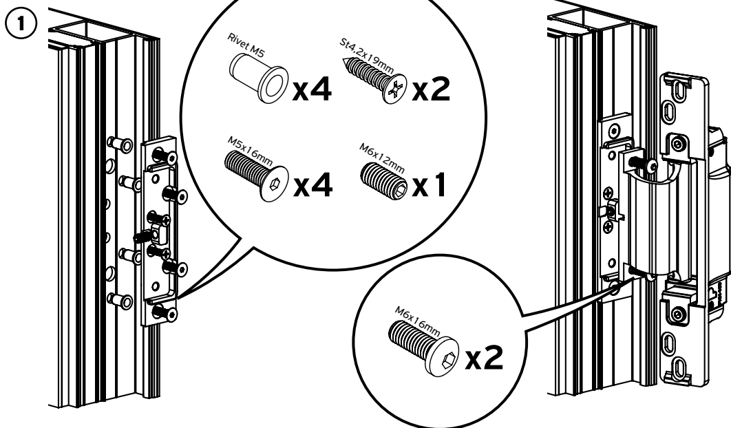
Installation of the hinge on the sash.
