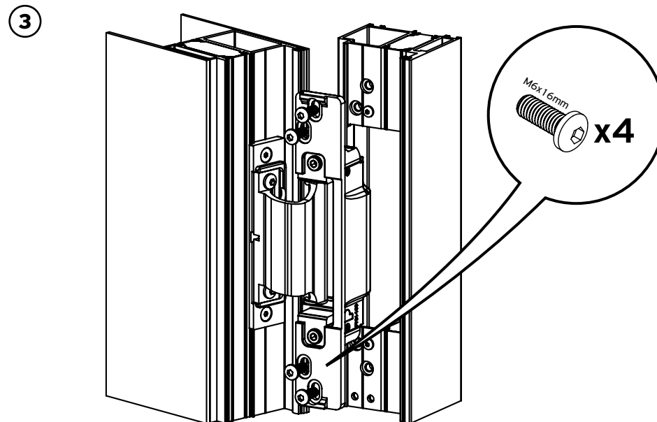
Installation of the hinge on the frame.
